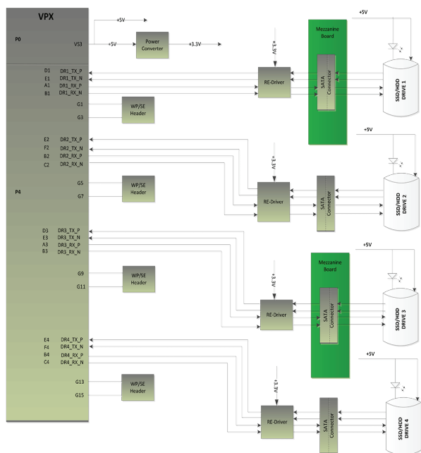
5632/5633 Block Diagram 6U VPX 6Gbps SATA Four Fixed Drives Storage Module
